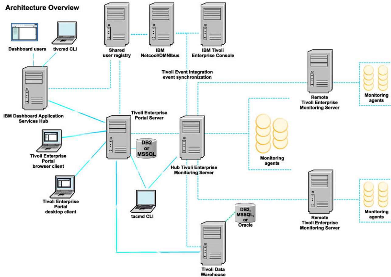
Figure 1. IBM Tivoli Monitoring environment
