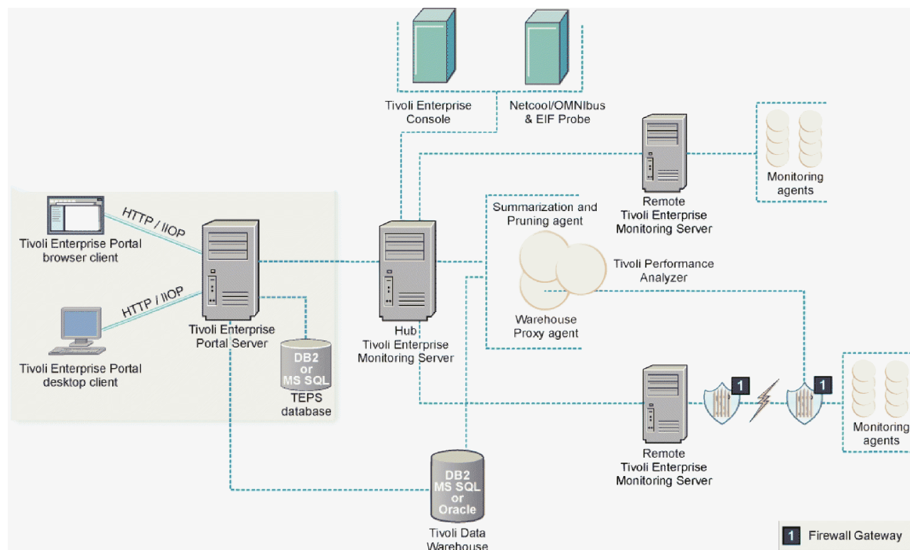
Figure 5. Tivoli Monitoring component architecture including firewall gateway
