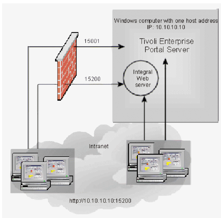
Figure 163. Intranet with integral Web server
