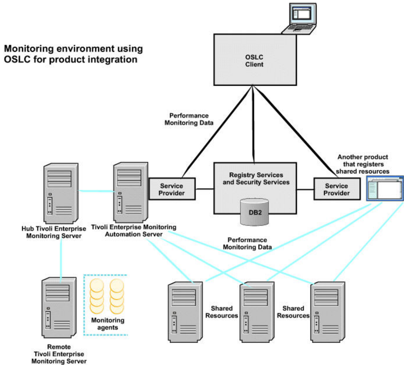
Figure 2. IBM Tivoli Monitoring environment using Open Services Lifecycle Collaboration for product integration
